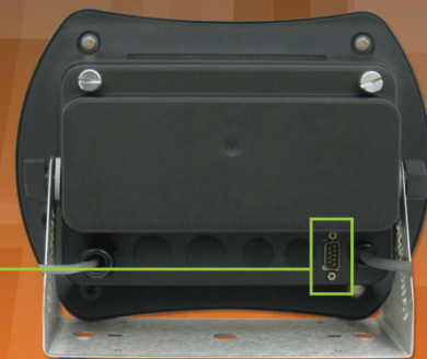
TS250 ABS Enclosure
